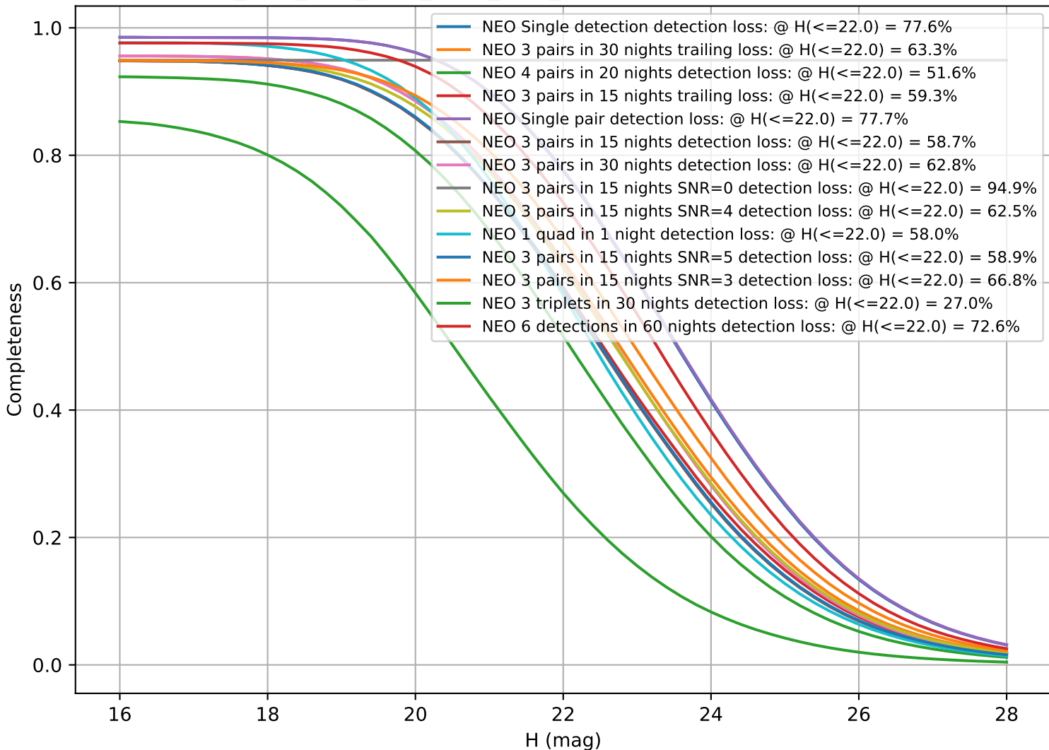
ddf_acor_sf15_lsf40_lsr50_v3.4_10yrs: CumulativeCompleteness
