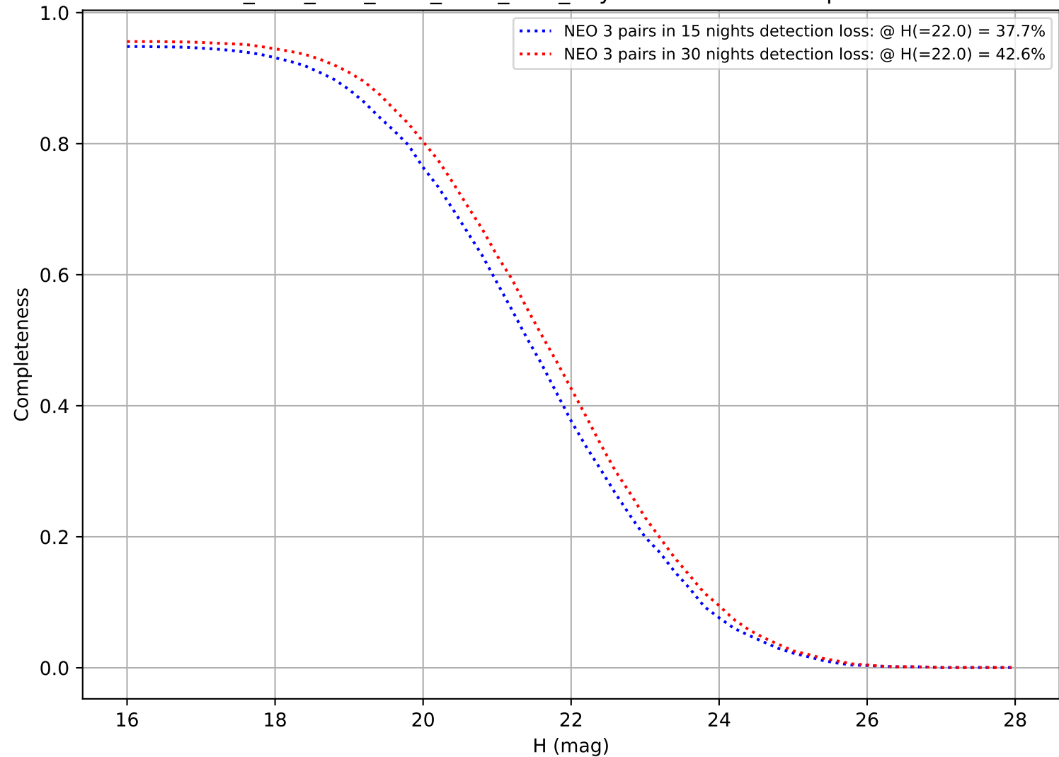
ddf_acor_sf15_lsf40_lsr50_v3.4_10yrs: DifferentialCompleteness
