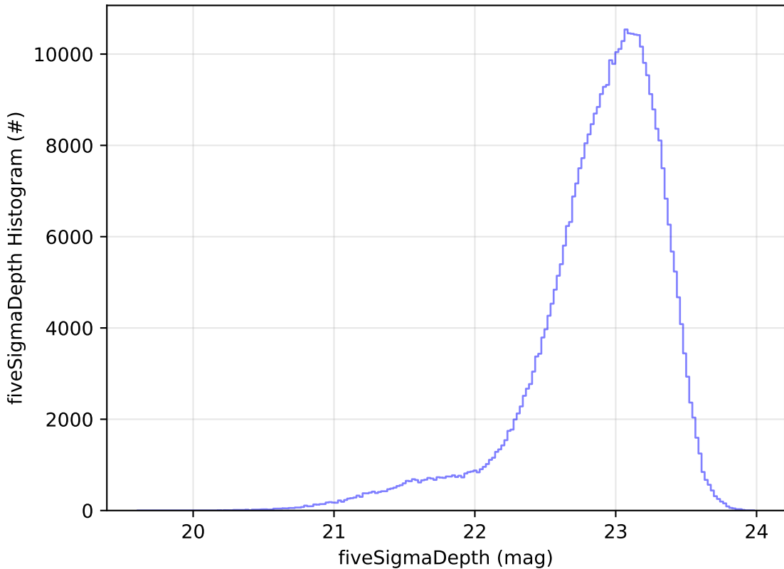
ddf_acor_sf15_lsf40_lsr50_v3.4_10yrs z: fiveSigmaDepth Histogram
