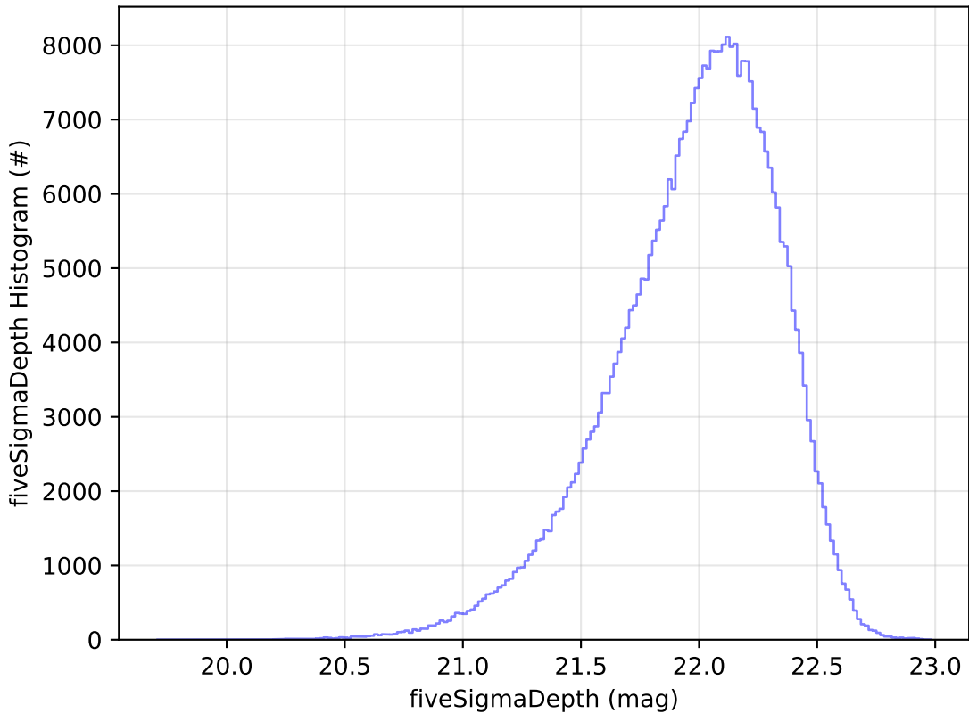
ddf_acor_sf15_lsf40_lsr50_v3.4_10yrs y: fiveSigmaDepth Histogram
