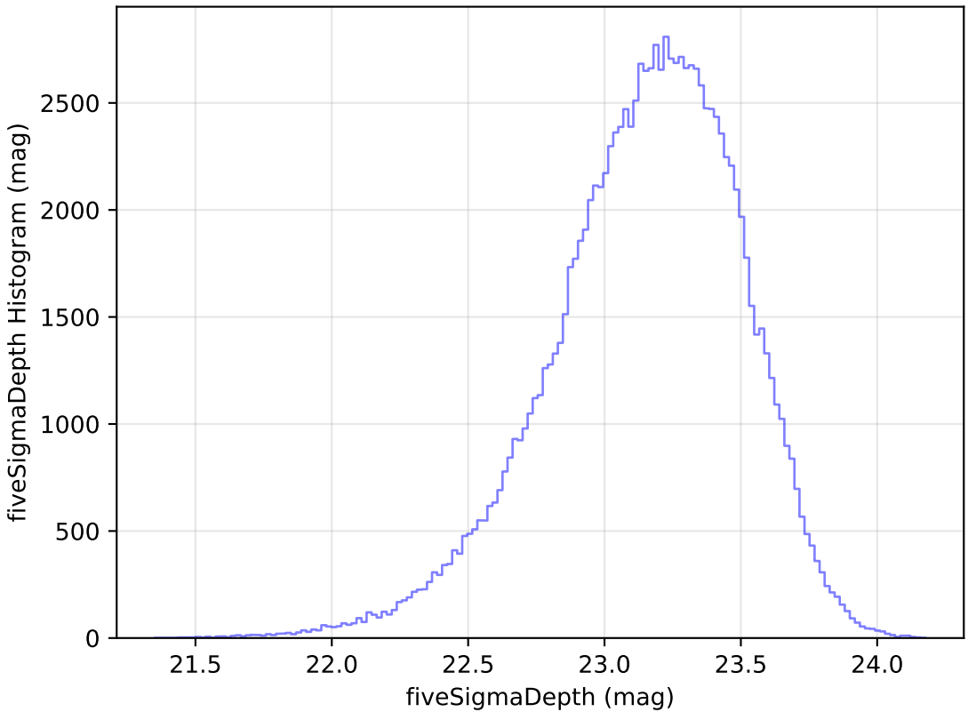
ddf_acor_sf15_lsf40_lsr50_v3.4_10yrs u: fiveSigmaDepth Histogram
