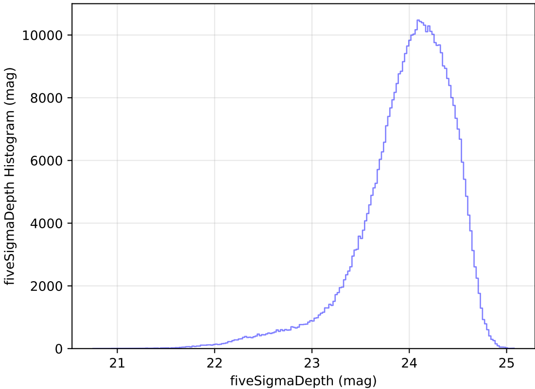
ddf_acor_sf15_lsf40_lsr50_v3.4_10yrs r: fiveSigmaDepth Histogram
