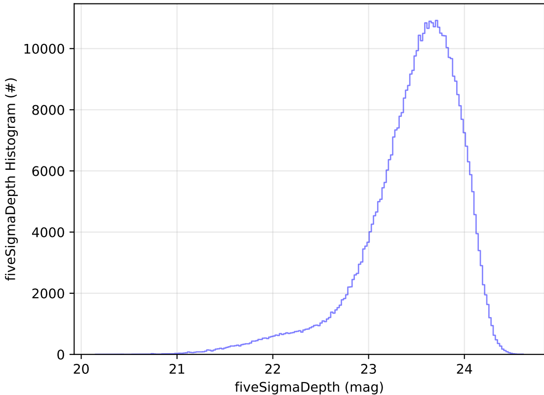
ddf_acor_sf15_lsf40_lsr50_v3.4_10yrs i: fiveSigmaDepth Histogram
