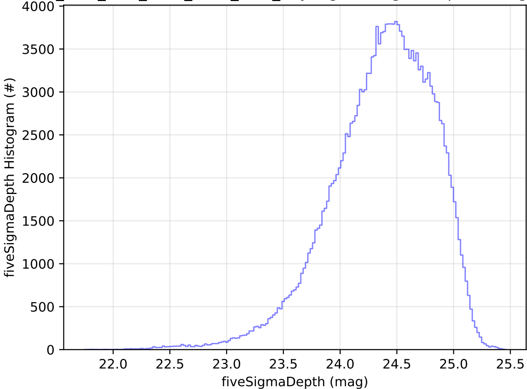
ddf_acor_sf15_lsf40_lsr50_v3.4_10yrs g: fiveSigmaDepth Histogram
