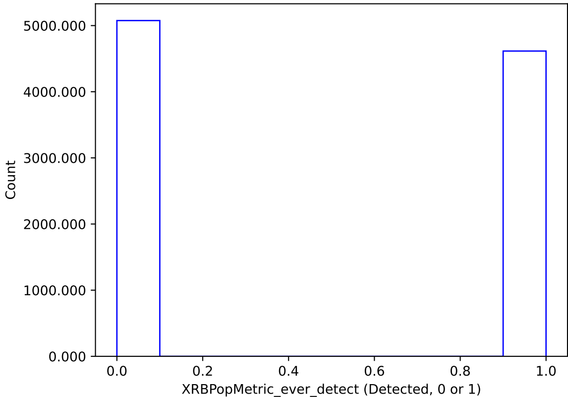
ddf_acor_sf15_lsf40_lsr50_v3.4_10yrs : XRBPoMetric_ever_detect
