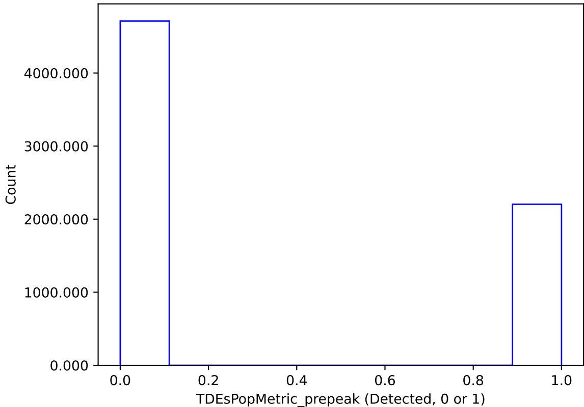
ddf_acor_sf15_lsf40_lsr50_v3.4_10yrs : TDEsPopMetric_prepeak
