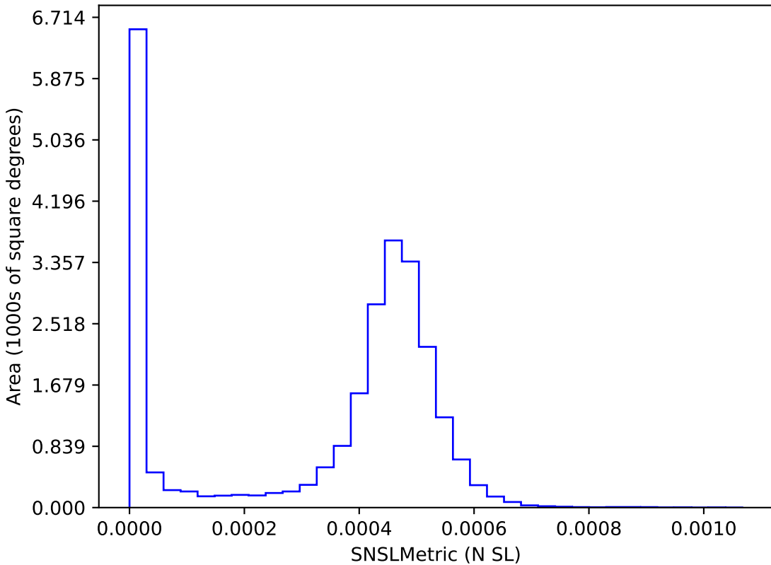
ddf_acor_sf15_lsf40_lsr50_v3.4_10yrs : SNSLMetric
