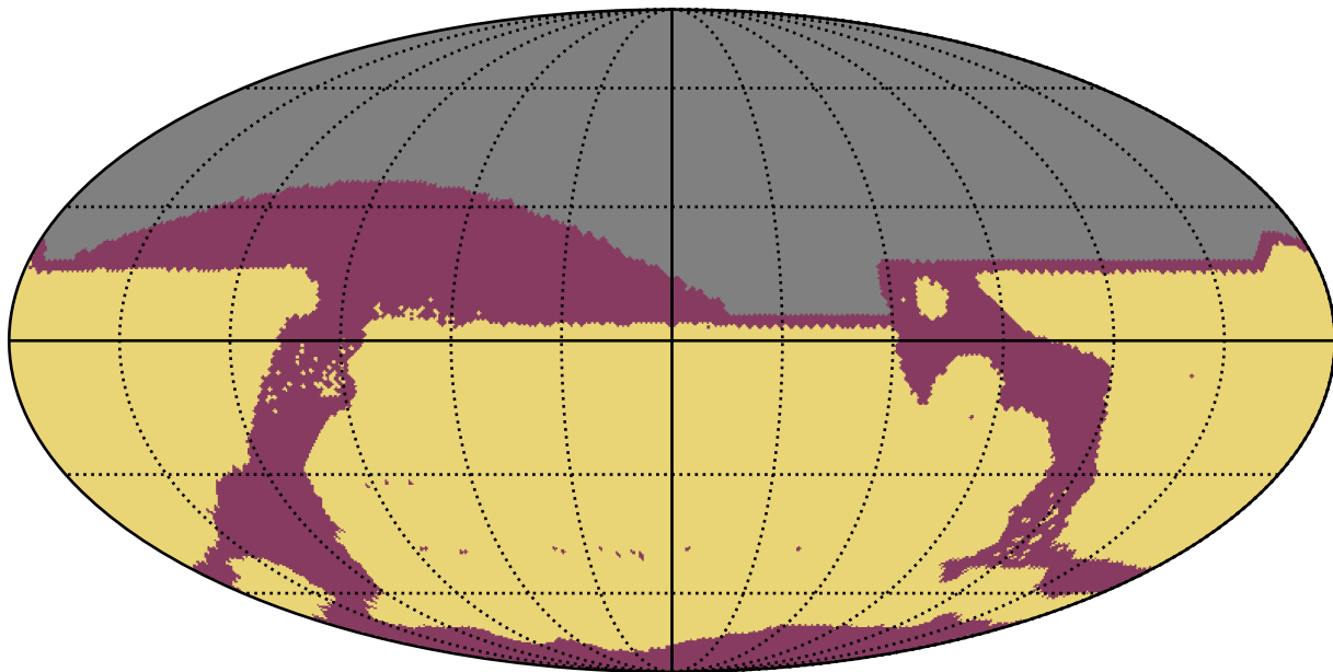
ddf_acor_sf15_lsf40_lsr50_v3.4_10yrs : RapidRevisits
