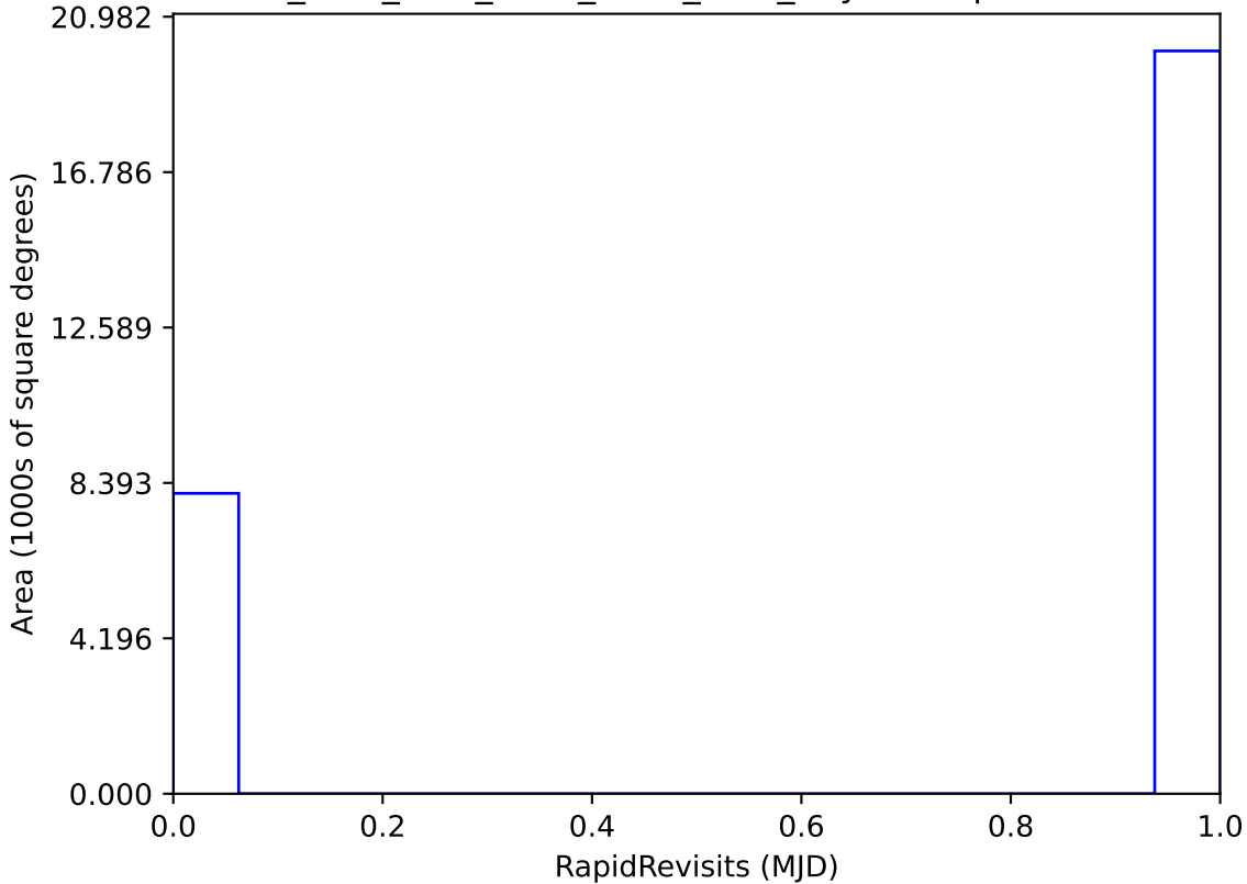
ddf_acor_sf15_lsf40_lsr50_v3.4_10yrs : RapidRevisits
