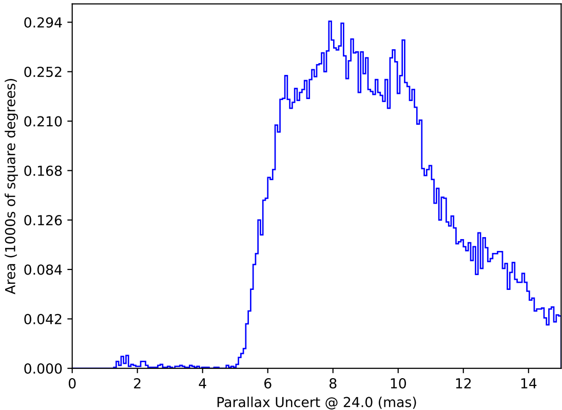
ddf_acor_sf15_lsf40_lsr50_v3.4_10yrs : Parallax Uncert @ 24.0
