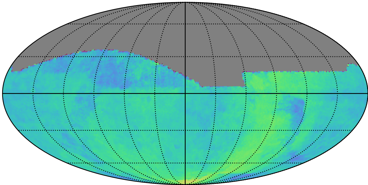
ddf_acor_sf15_lsf40_lsr50_v3.4_10yrs : Parallax Coverage @ 24.0
