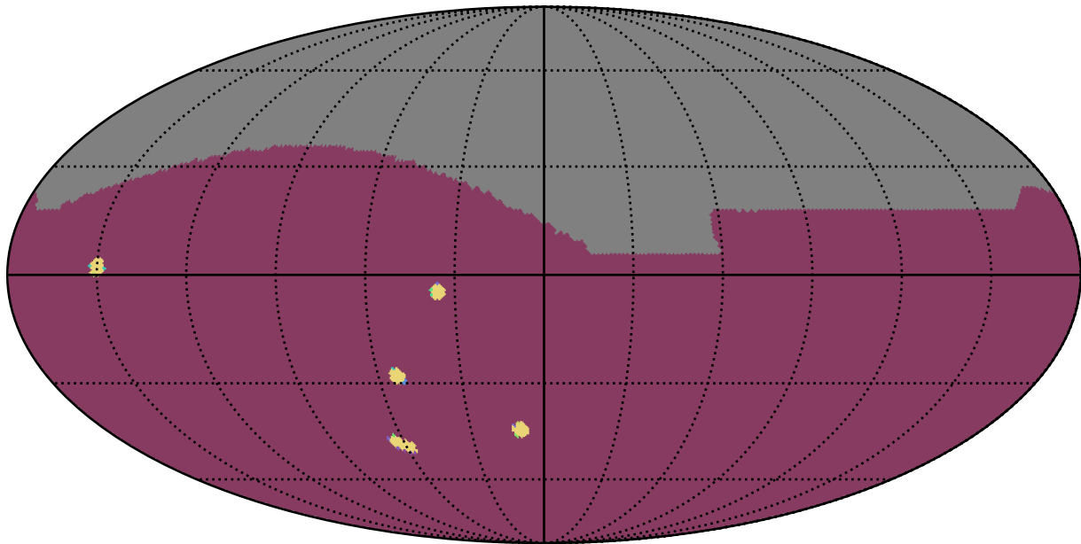
ddf_acor_sf15_lsf40_lsr50_v3.4_10yrs : NumberOfQuickRevisits
