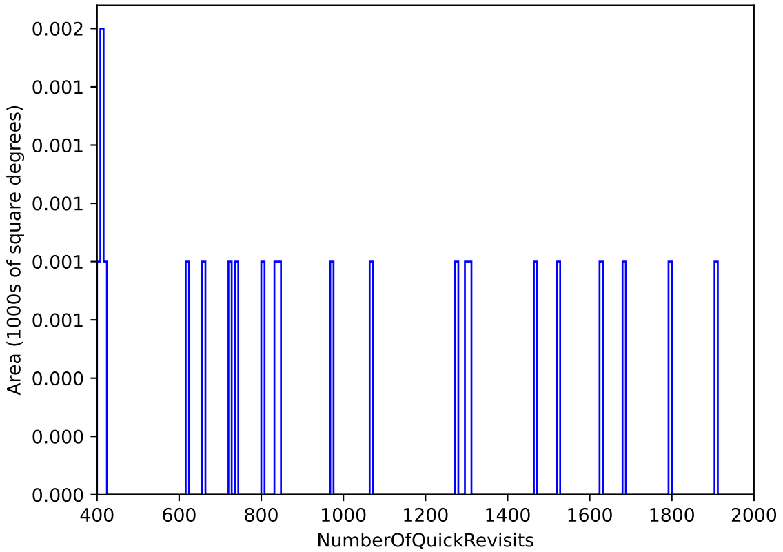
ddf_acor_sf15_lsf40_lsr50_v3.4_10yrs : NumberOfQuickRevisits
