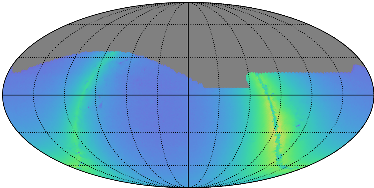
ddf_acor_sf15_lsf40_lsr50_v3.4_10yrs r: Nstars_no_crowding
