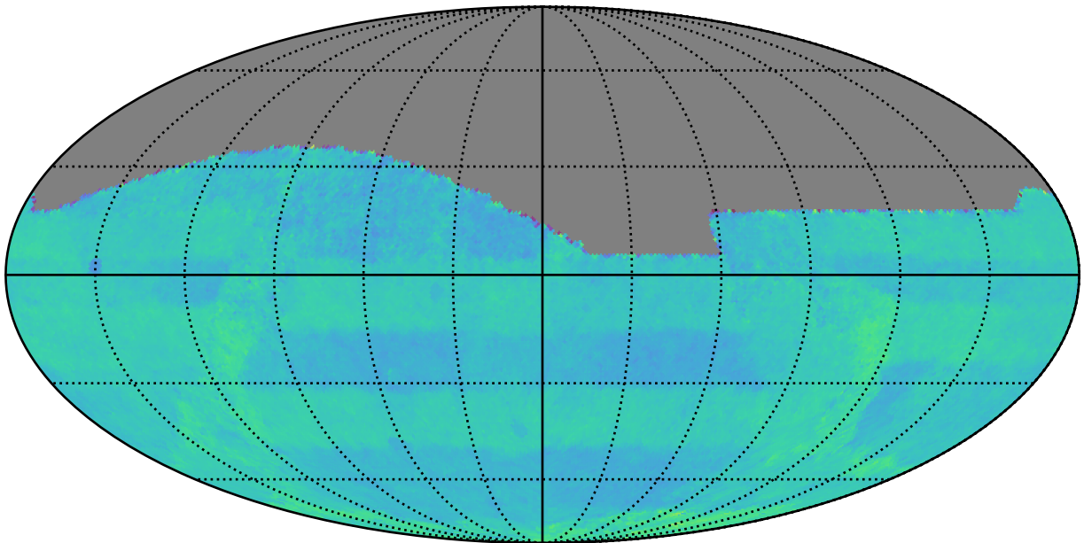
ddf_acor_sf15_lsf40_lsr50_v3.4_10yrs : Normalized Proper Motion Uncert @ 24.0
