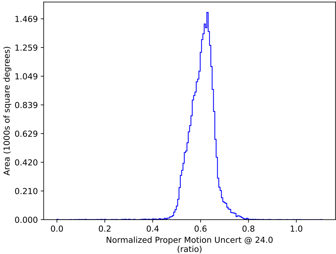
ddf_acor_sf15_lsf40_lsr50_v3.4_10yrs : Normalized Proper Motion Uncert @ 24.0
