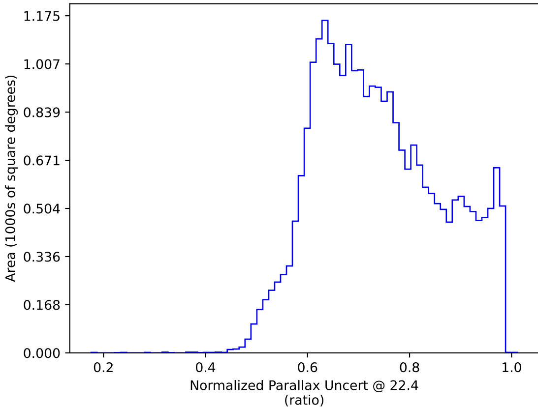
ddf_acor_sf15_lsf40_lsr50_v3.4_10yrs : Normalized Parallax Uncert @ 22.4
