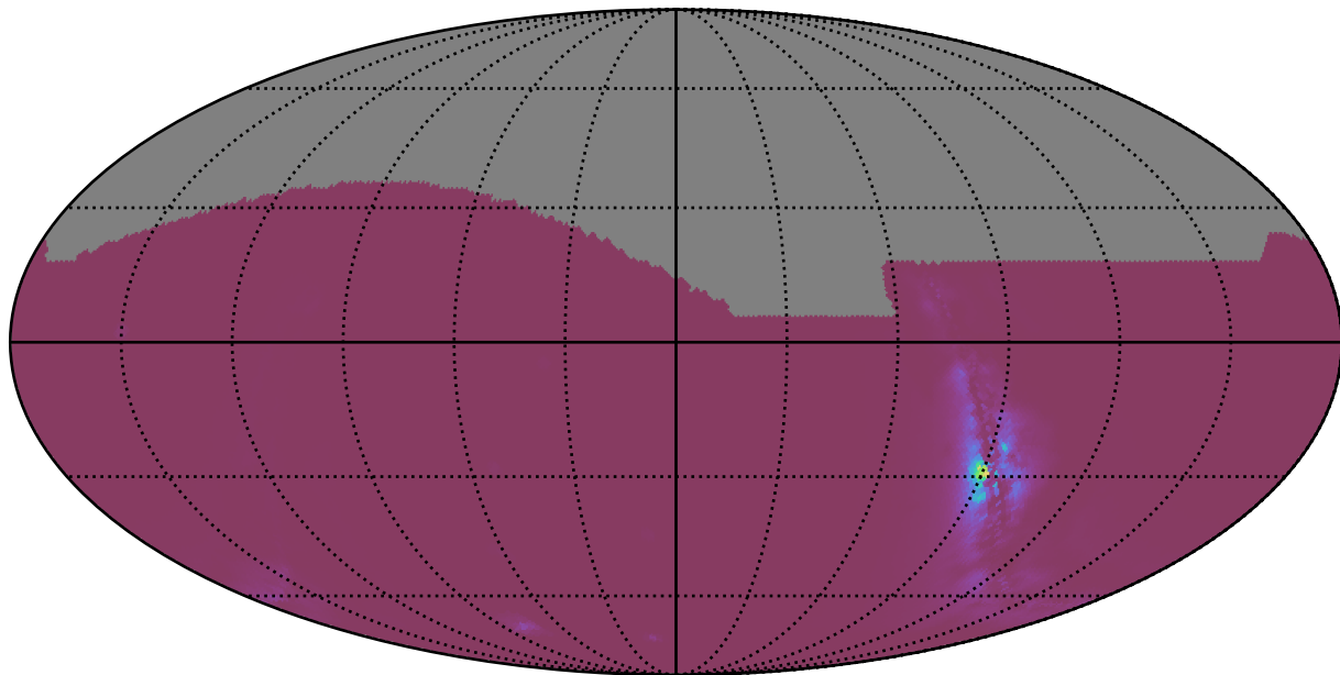
ddf_acor_sf15_lsf40_lsr50_v3.4_10yrs : NlcPoints
