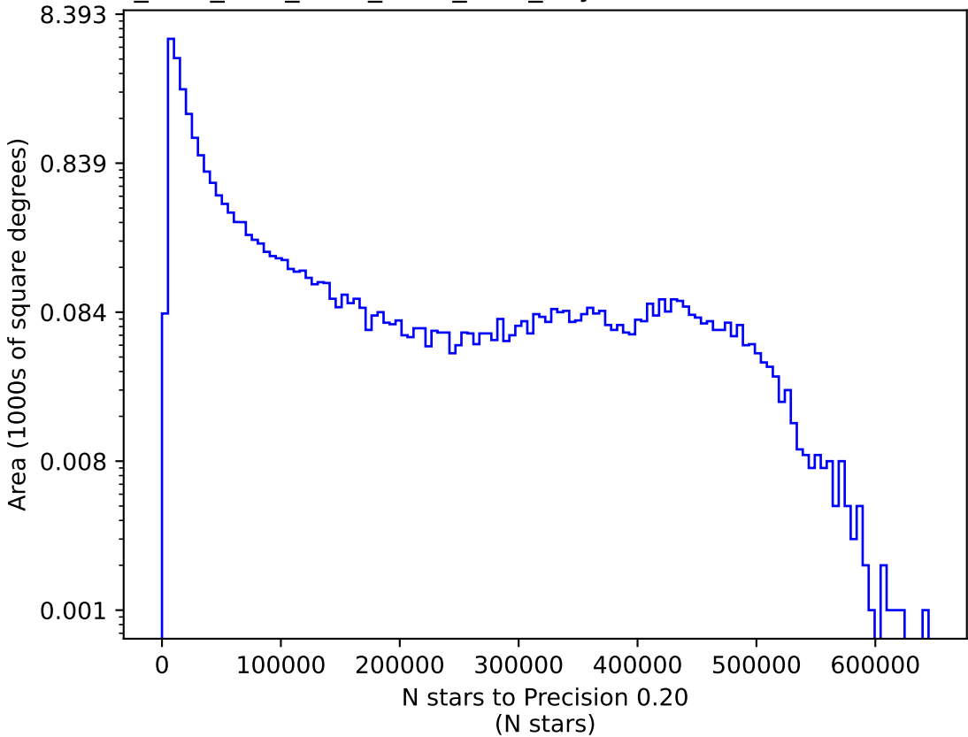
ddf_acor_sf15_lsf40_lsr50_v3.4_10yrs i: N stars to Precision 0.20
