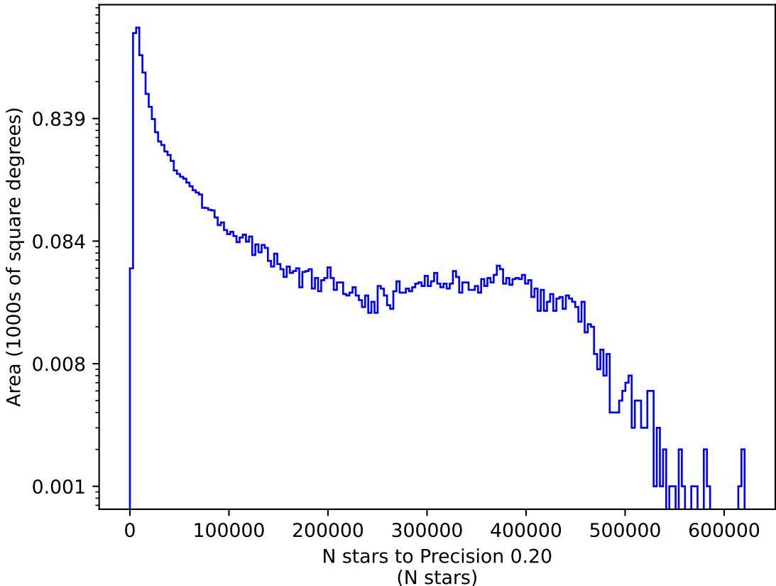
ddf_acor_sf15_lsf40_lsr50_v3.4_10yrs g: N stars to Precision 0.20
