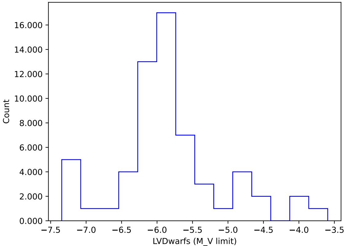
ddf_acor_sf15_lsf40_lsr50_v3.4_10yrs gi: LVDwarfs
