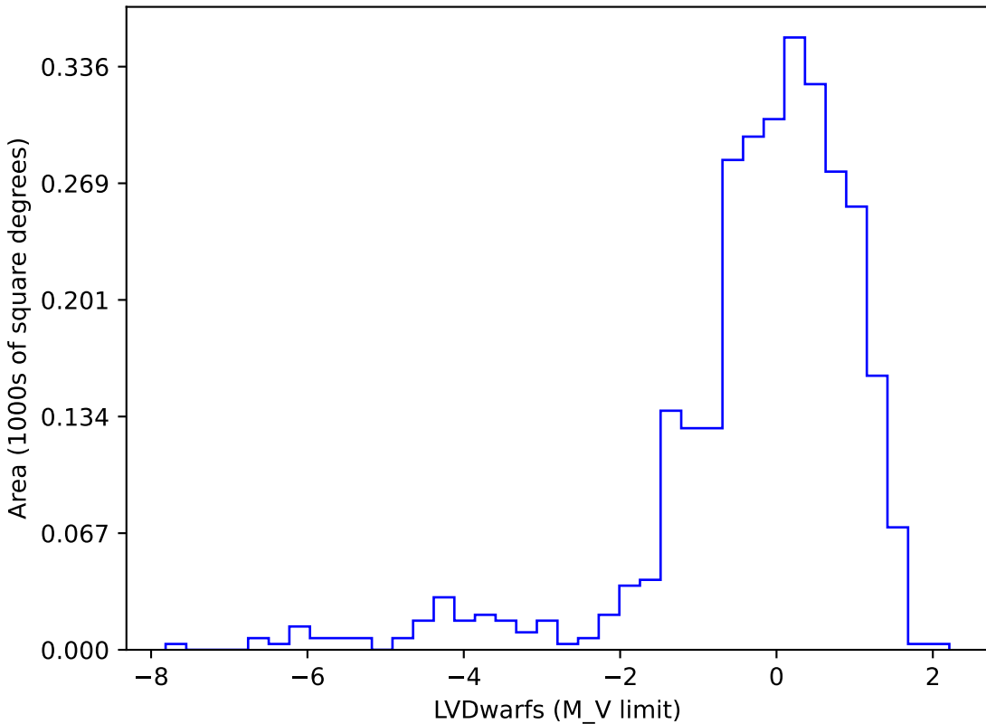
ddf_acor_sf15_lsf40_lsr50_v3.4_10yrs gi SCP: LVDwarfs
