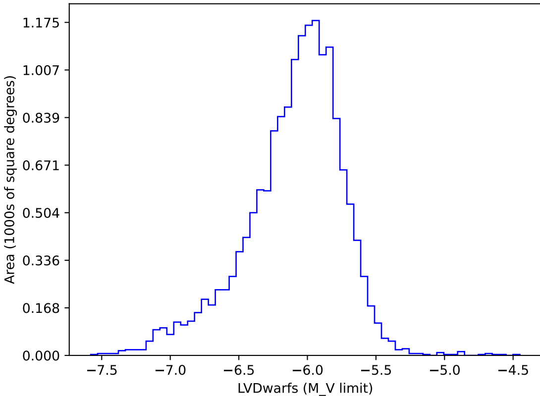
ddf_acor_sf15_lsf40_lsr50_v3.4_10yrs gi: LVDwarfs
