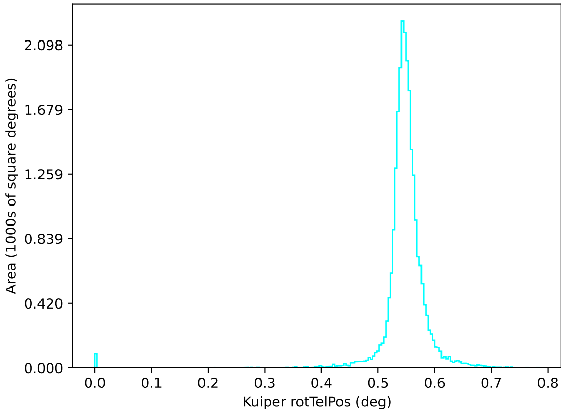
ddf_acor_sf15_ls40_lsr50_v3.4_10yrs u: Kuiper rotTelPos
