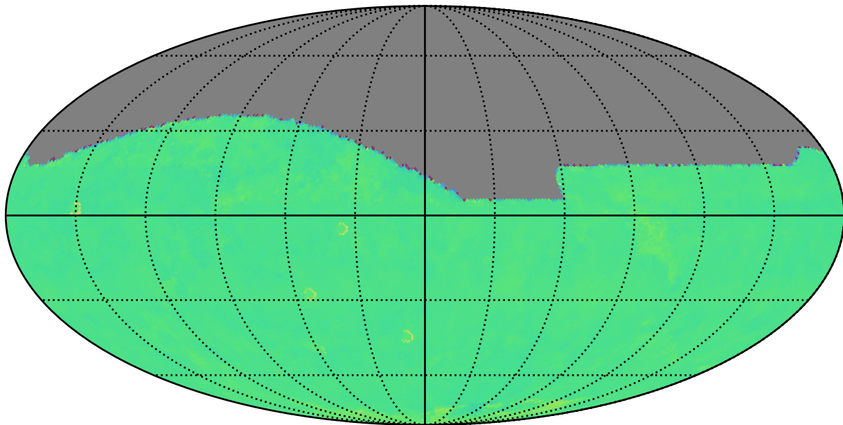
ddf_acor_sf15_lsf40_lsr50_v3.4_10yrs r: Kuiper rotTelPos
