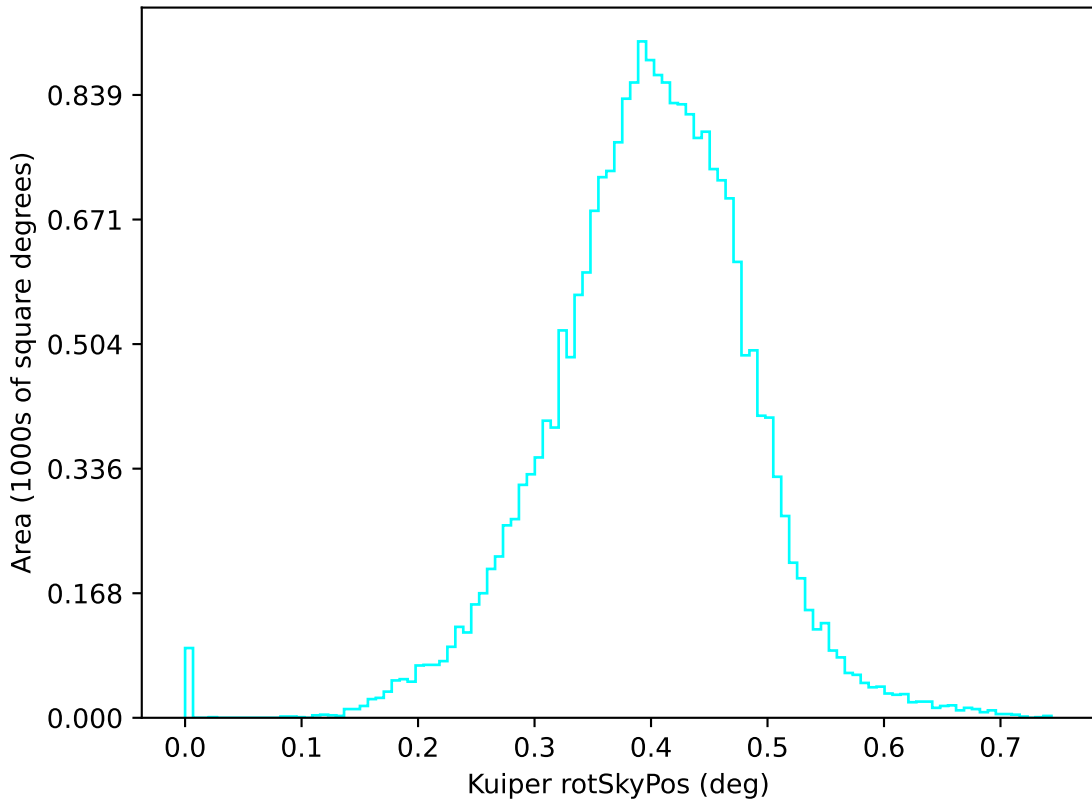
ddf_acor_sf15_lsf40_lsr50_v3.4_10yrs u: Kuiper rotSkyPos
