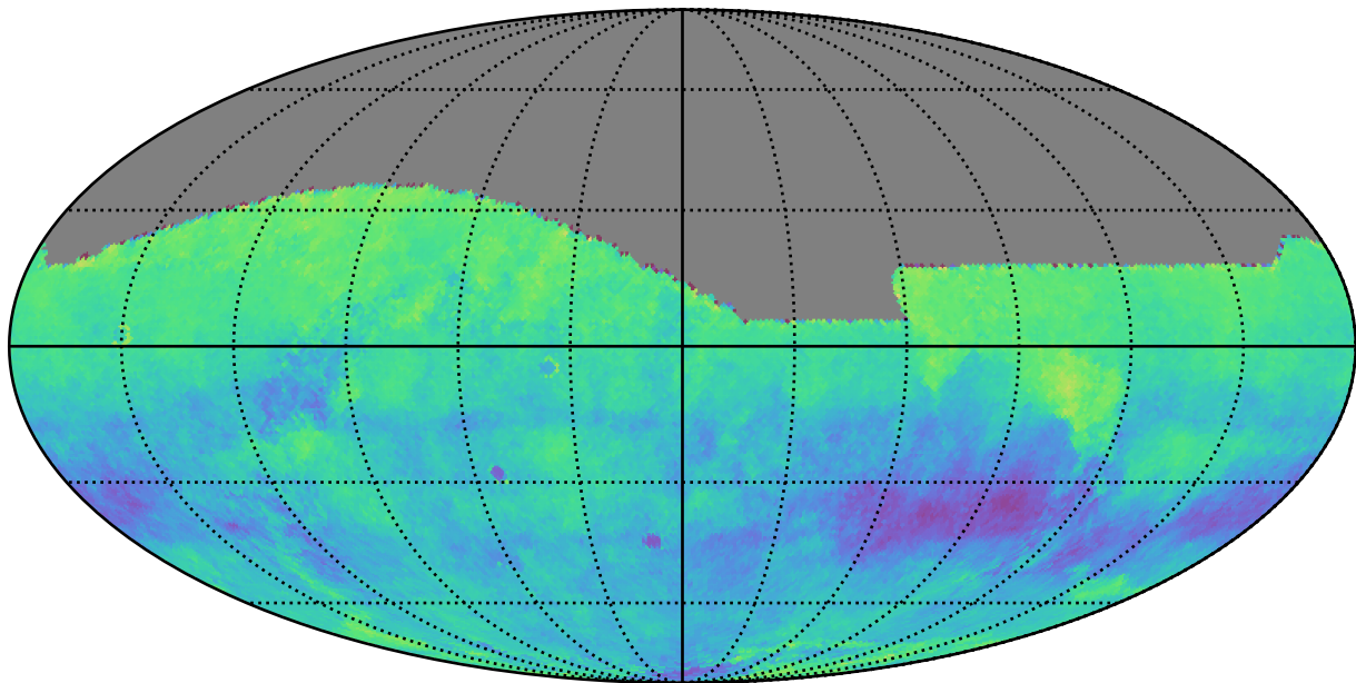
ddf_acor_sf15_lsf40_lsr50_v3.4_10yrs r: Kuiper rotSkyPos
