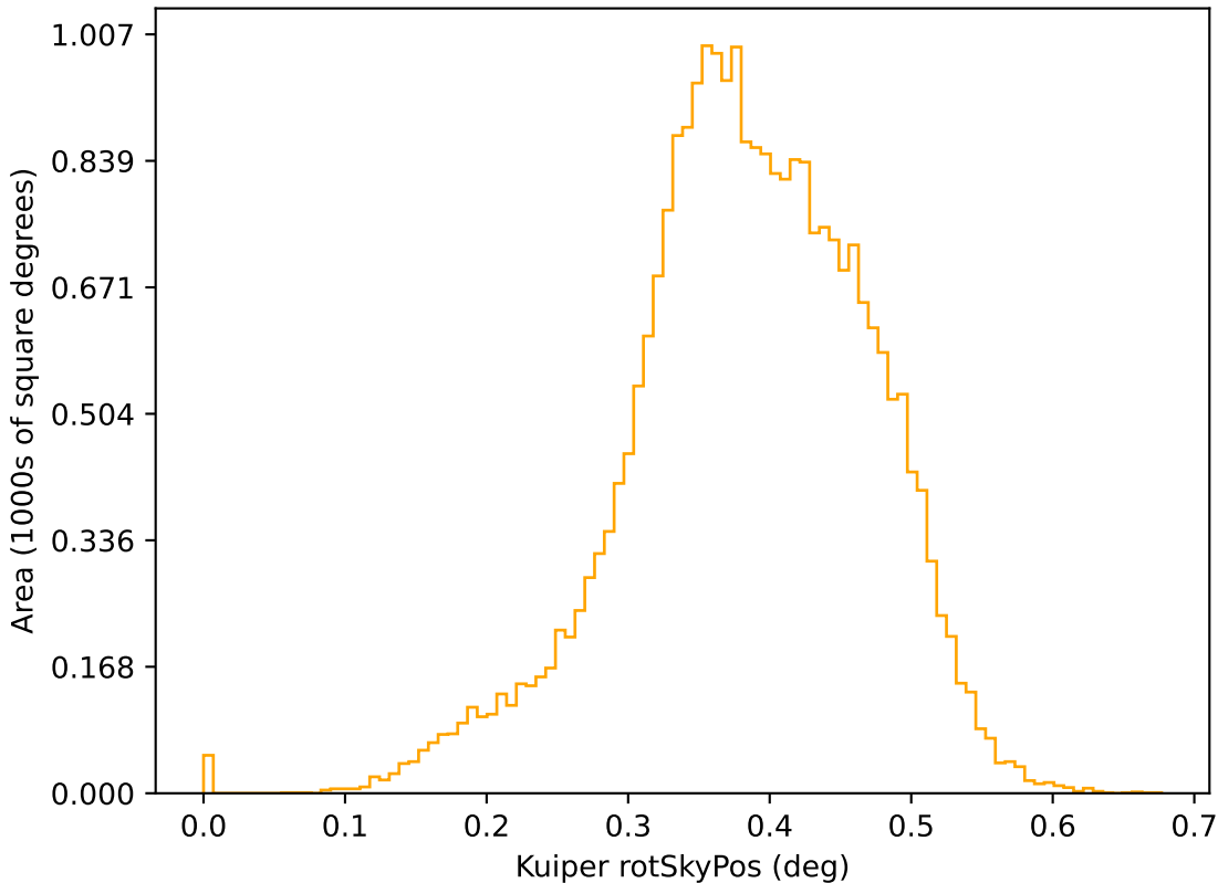
ddf_acor_sf15_lsf40_lsr50_v3.4_10yrs r: Kuiper rotSkyPos
