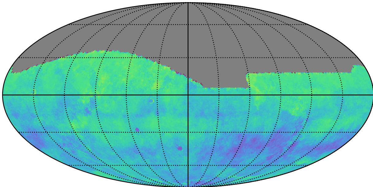
ddf_acor_sf15_lsf40_lsr50_v3.4_10yrs i: Kuiper rotSkyPos
