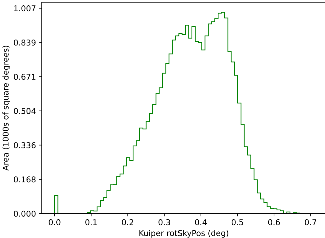
ddf_acor_sf15_lsf40_lsr50_v3.4_10yrs g: Kuiper rotSkyPos
