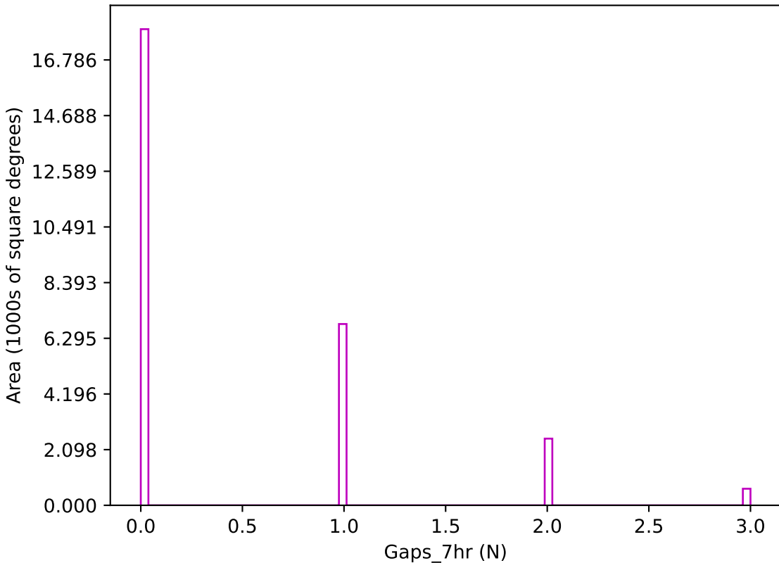
ddf_acor_sf15_ls40_lsr50_v3.4_10yrs z band: Gaps_7hr
