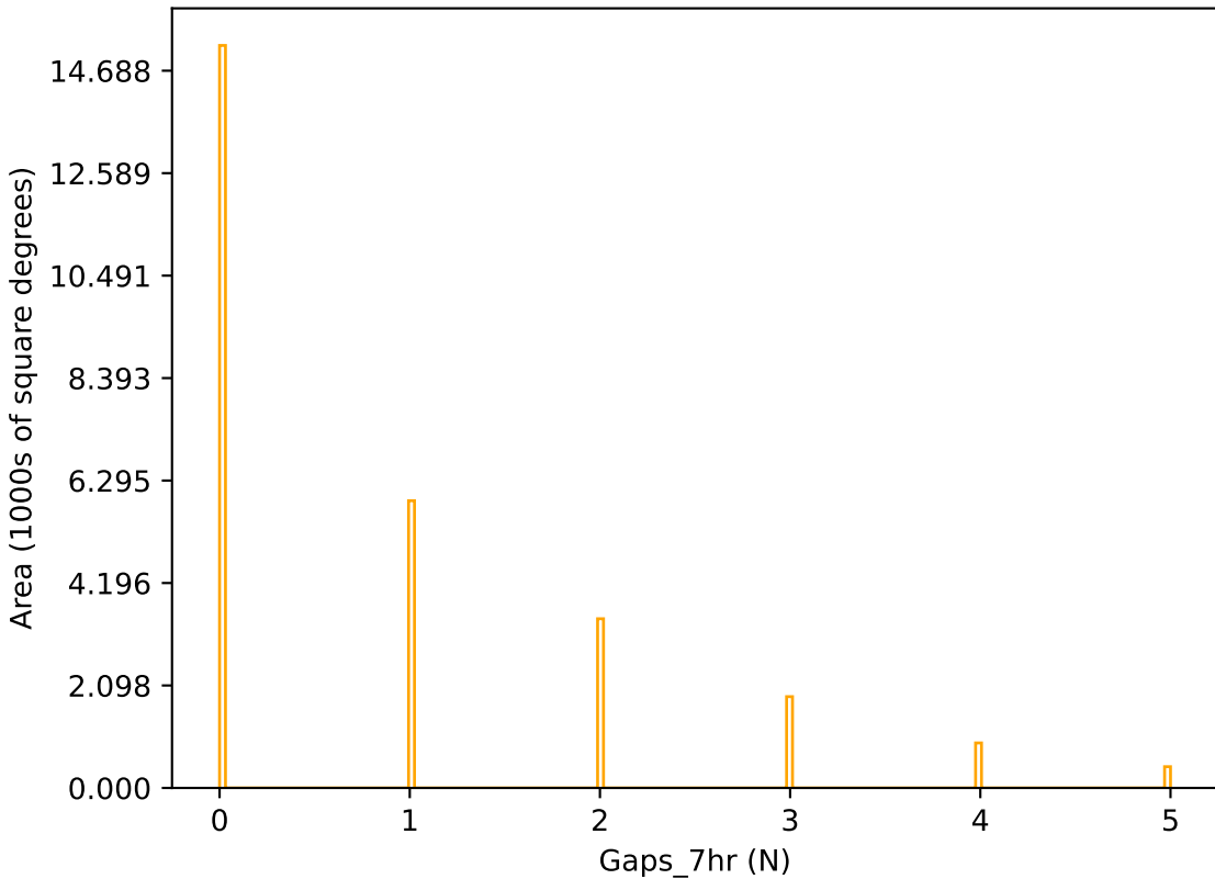
ddf_acor_sf15_lsf40_lsr50_v3.4_10yrs r band: Gaps_7hr
