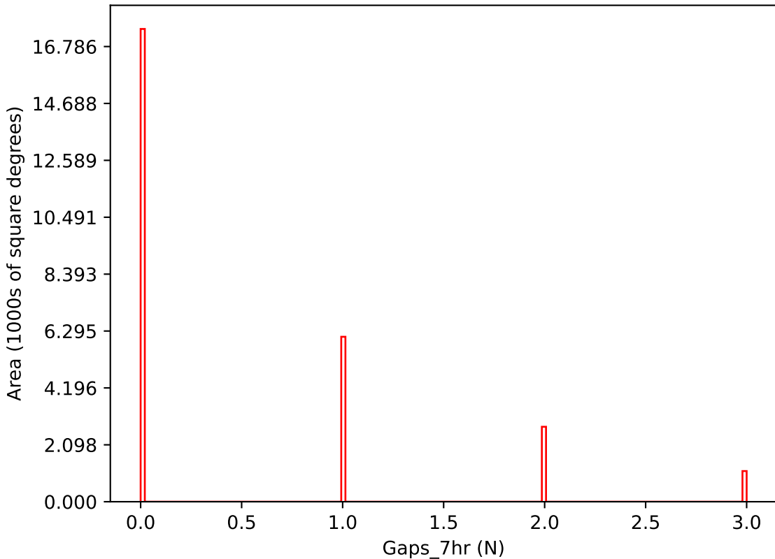
ddf_acor_sf15_lsf40_lsr50_v3.4_10yrs i band: Gaps_7hr
