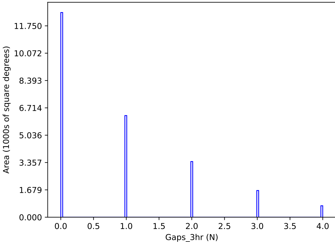
ddf_acor_sf15_lsf40_lsr50_v3.4_10yrs y band: Gaps_3hr
