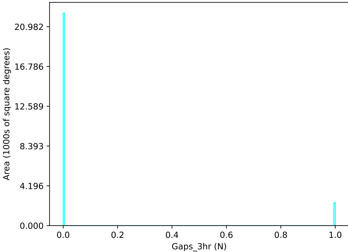
ddf_acor_sf15_lsf40_lsr50_v3.4_10yrs u band: Gaps_3hr
