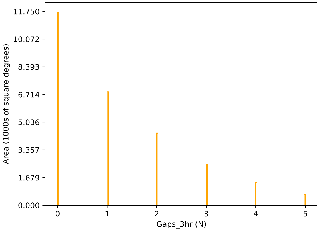
ddf_acor_sf15_lsf40_lsr50_v3.4_10yrs r band: Gaps_3hr
