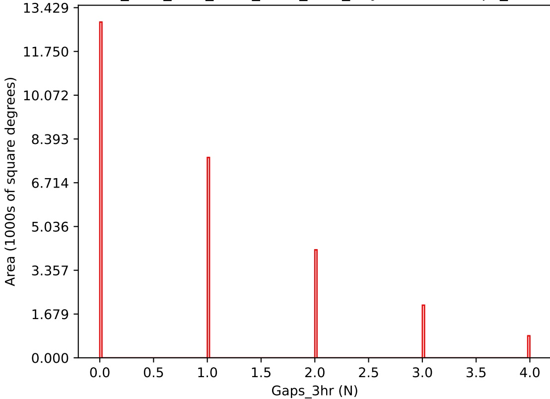
ddf_acor_sf15_lsf40_lsr50_v3.4_10yrs i band: Gaps_3hr
