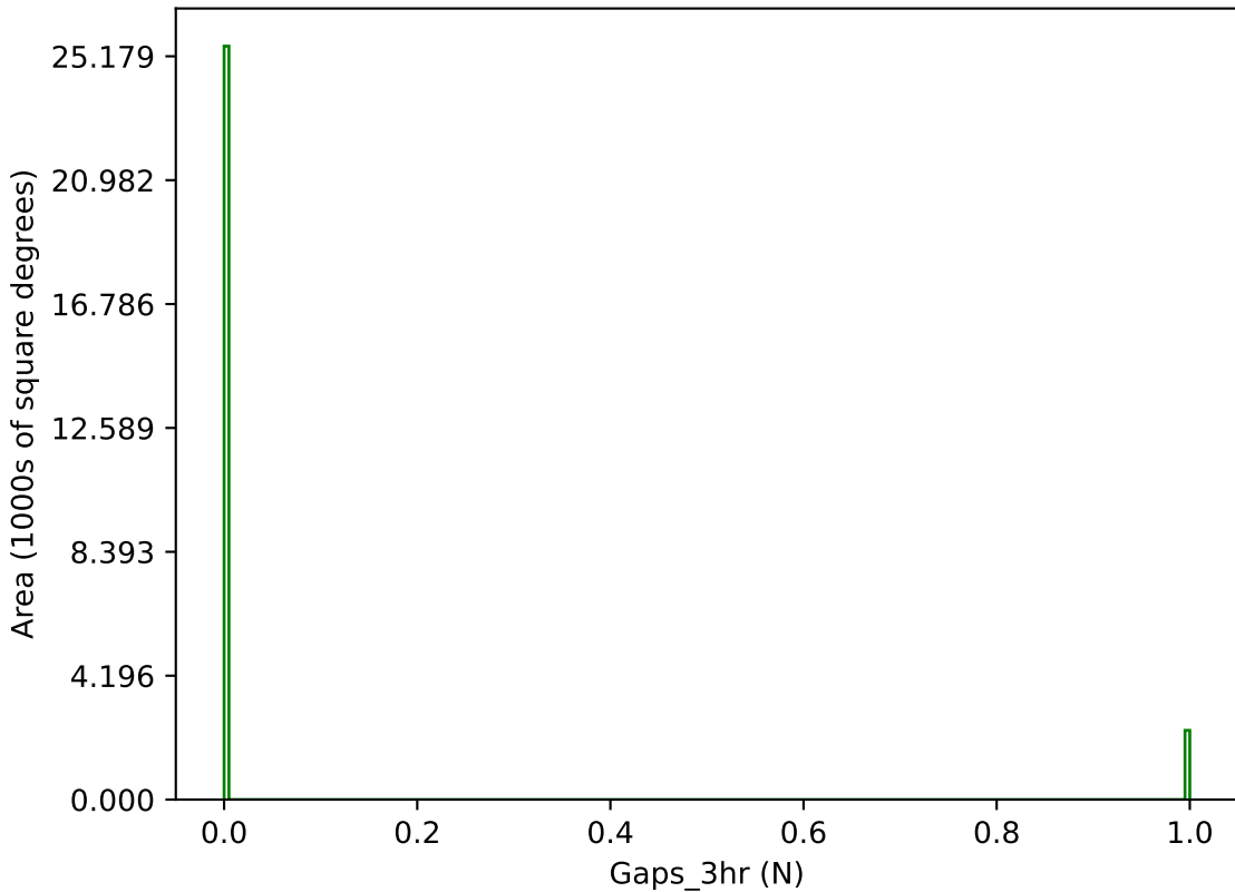
ddf_acor_sf15_lsf40_lsr50_v3.4_10yrs g band: Gaps_3hr
