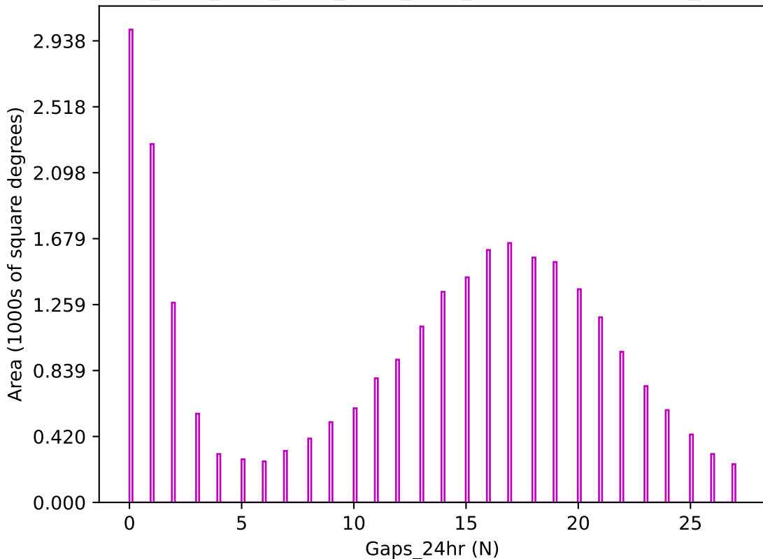
ddf_acor_sf15_lsf40_lsr50_v3.4_10yrs z band: Gaps_24hr
