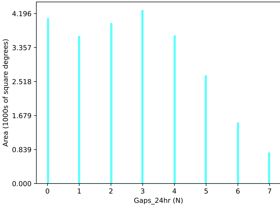
ddf_acor_sf15_lsf40_lsr50_v3.4_10yrs u band: Gaps_24hr
