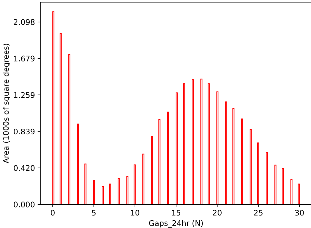
ddf_acor_sf15_lsf40_lsr50_v3.4_10yrs i band: Gaps_24hr
