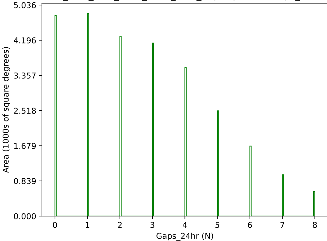
ddf_acor_sf15_lsf40_lsr50_v3.4_10yrs g band: Gaps_24hr
