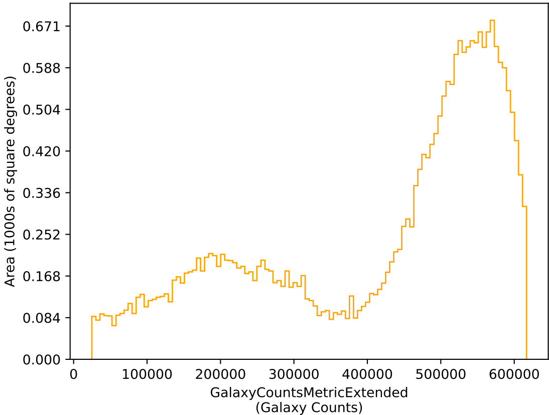
ddf_acor_sf15_lsf40_lsr50_v3.4_10yrs r: GalaxyCountsMetricExtended
