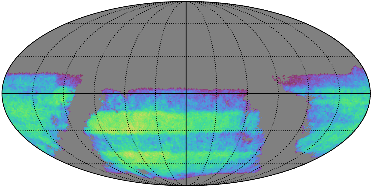
ddf_acor_sf15_lsf40_lsr50_v3.4_10yrs i band non-DD year 3: ExgalM5WithCuts
