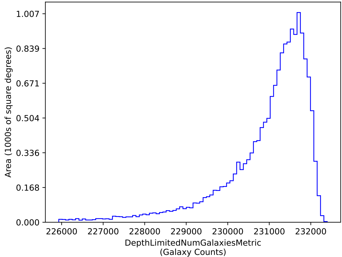
ddf_acor_sf15_lsf40_lsr50_v3.4_10yrs i band galaxies non-DD: DepthLimitedNumGalaxiesMetric
