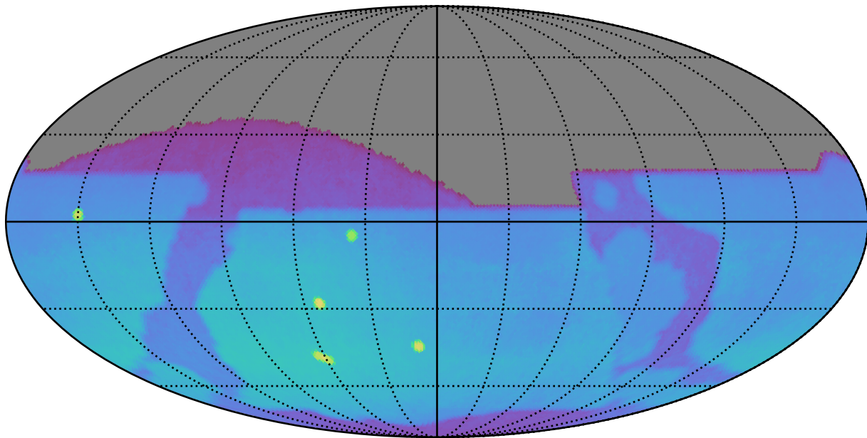
ddf_acor_sf15_lsf40_lsr50_v3.4_10yrs : Brown Dwarf, L7
